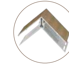
2PC 2.5" OUTSIDE CORNER TRIM (LARGE FACE) USE WITH PANEL LENGTHS GREATER THAN 20'
