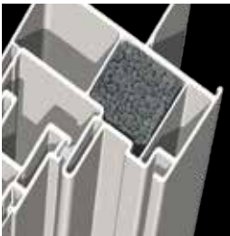
BarrierXP iE features carbonized foam liners in select masterframe channels for increased energy efficiency.
