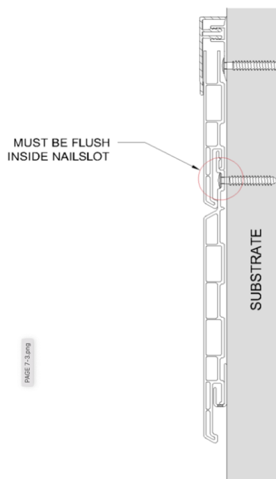
CORRECT INSTALL
